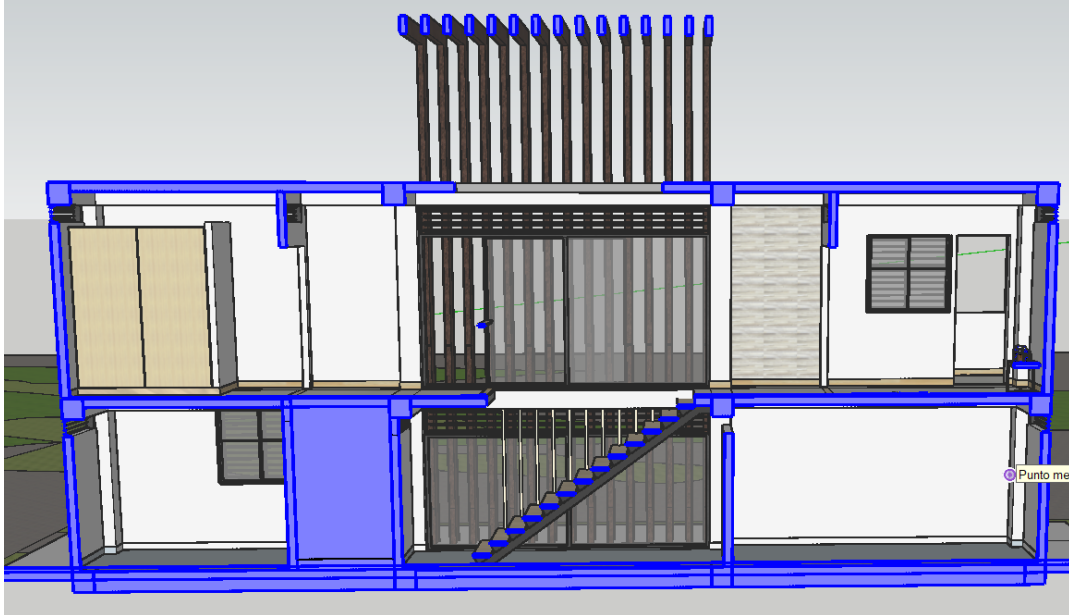
Corte transversal general
